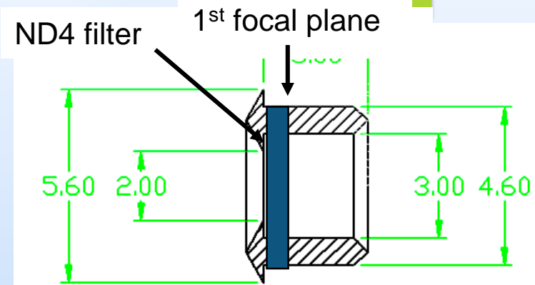
Fig. Crosssection of an occulting mask
